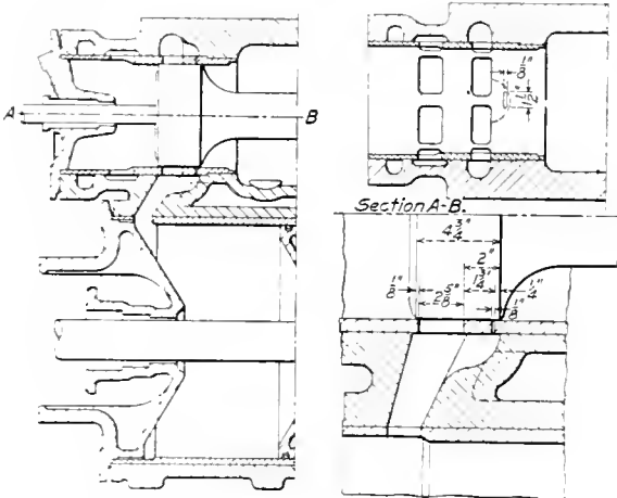
Valve Chamber with Auxillary Starting Ports
